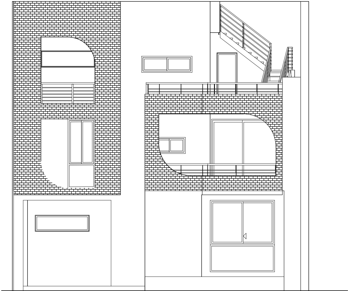
WEST ELEVATION
